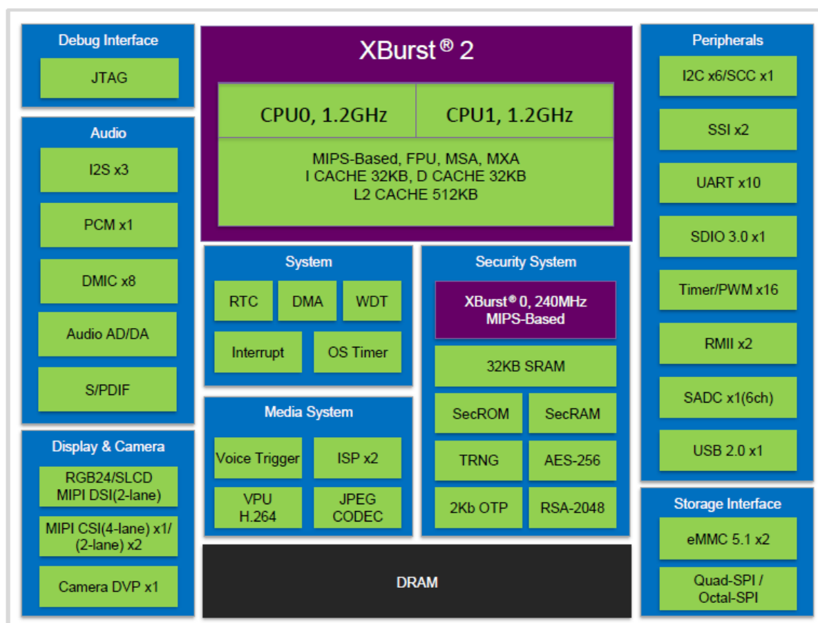
Figure 1-1 X2100/X2100L Diagram
